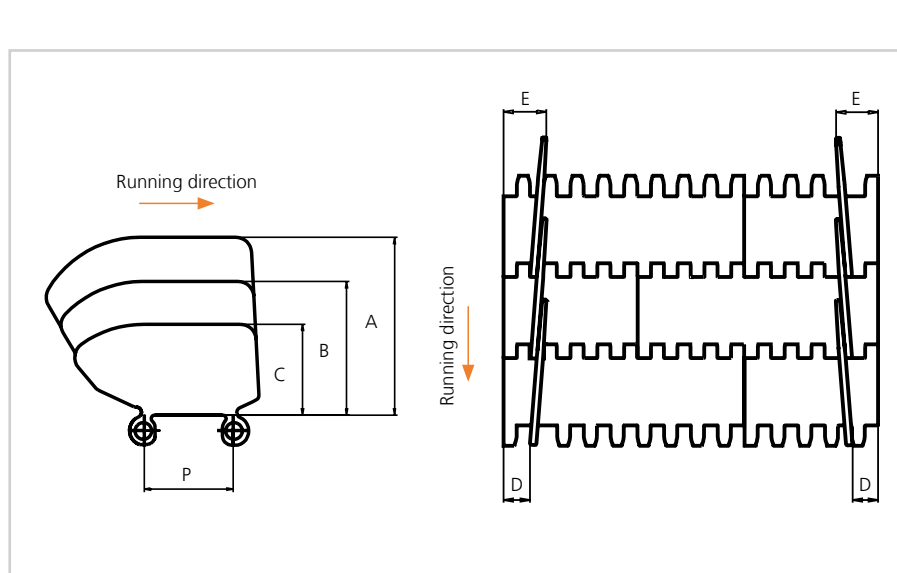
uni MPB Side Guard
