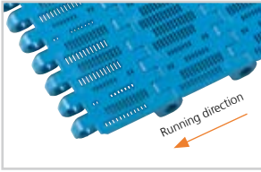
uni BLB Surface opening 18%, Top
