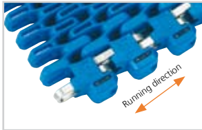
uni Flex SNB W Surface opening 55%
